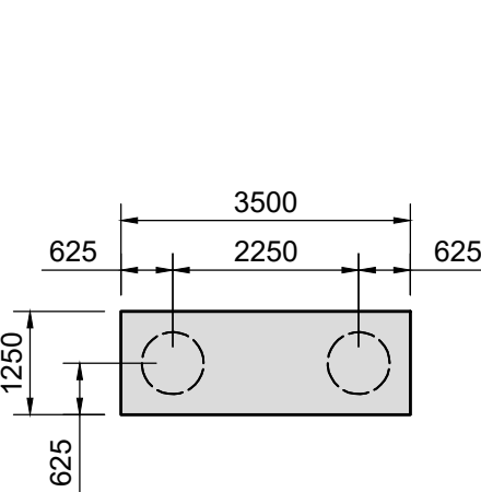
PILE CAP - PC1 SCALE 1:100
