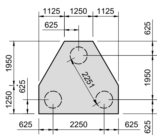
PILE CAP - PC2 SCALE 1:100
