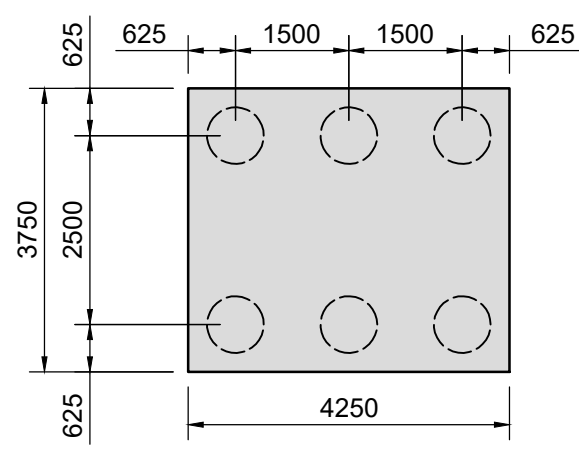
PILE CAP - PC8 SCALE 1:100
