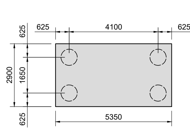
PILE CAP - PC9 SCALE 1:100
