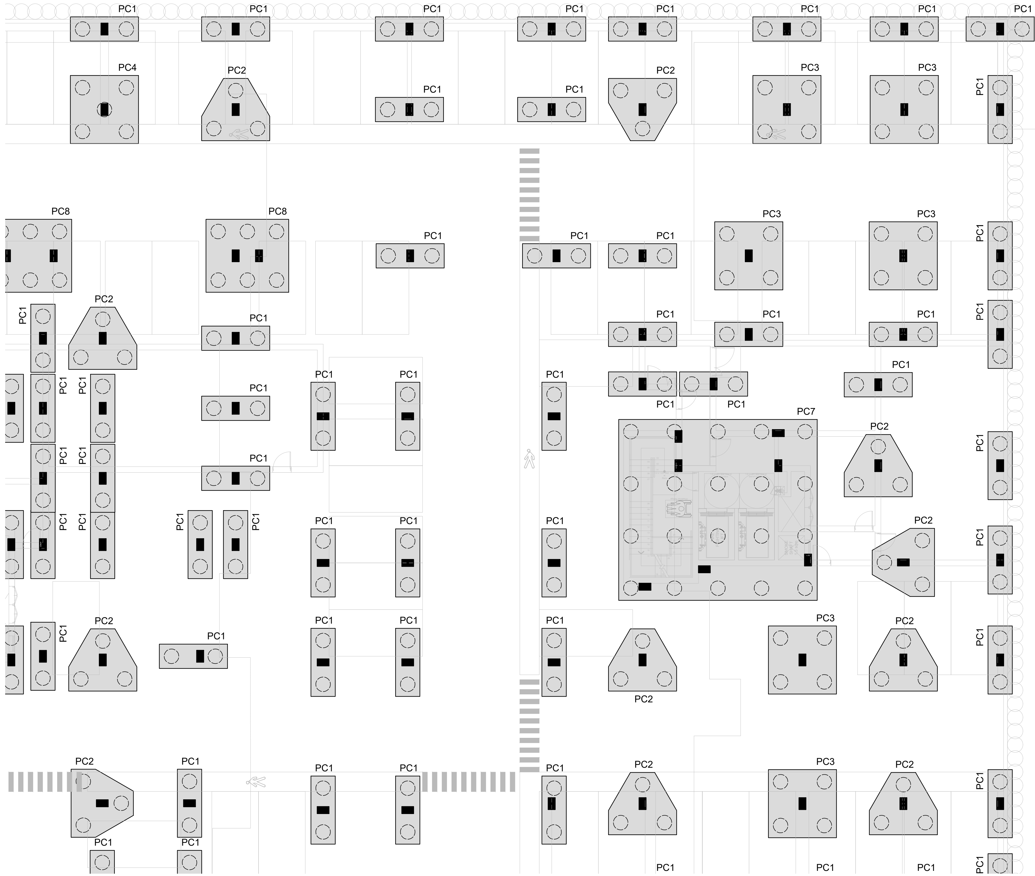
PILE CAP LAYOUT - ZONE 2 SCALE 1:100
